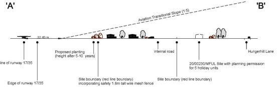
Site Section
